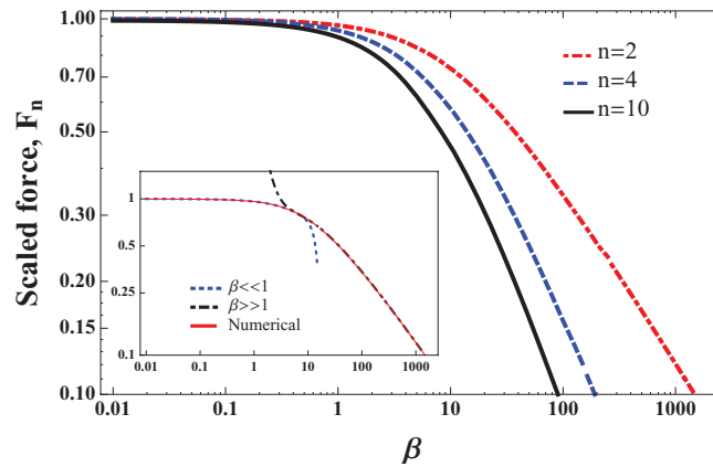
FIG. 3. The force on the particle as a function of \beta = 12k\ell_n^2/\delta^3 , calculated using Eq. (17), for different particle shapes. Shown in the inset are the asymptotic solutions for the sphere, n = 2 , given by Eqs. (30) and (32) in the case of small and large \beta , respectively, and compared to the numerical solution of Eq. (14).
