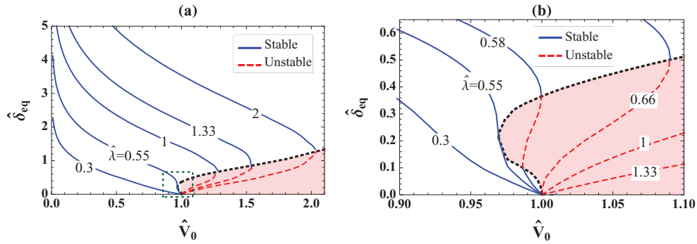
FIG. 7. The equilibrium separation distance, \delta_{eq} , of a sphere near a charged, permeable surface, in the presence of a background permeation of the surrounding fluid. (a) Calculations made using a steady-state Eq. (41) for various values of \hat{\lambda} , the scaled electric-double-layer thickness, and \hat{V}_0 , representing the viscous lubrication forces and electrostatic repulsion. (b) Same as (a), magnification of the region near \hat{V}_0 = 1 (dashed rectangle in (a)), showing the possibility of three equilibria. The calculations show regions of stable and unstable (shaded, red online) equilibria. The value \hat{\lambda} \approx 0.55 signifies the transition from a region of a single, stable equilibrium to a region of three equilibria, followed by a transition to two equilibria at \hat{\lambda} = 2/3 .
