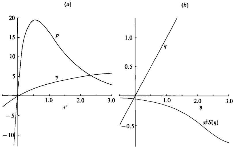
FIGURE 11. (a) Graphs of p(\tau') and \eta(\tau') for \alpha = 50 . p(\tau') has a maximum of (8\sqrt{3}\alpha+9)/36 at \tau' = \frac{1}{2} \ln 3 . (b) Graph of \alpha^{1/3}S(\eta) for comparison with \eta itself, for \alpha = 50 .
